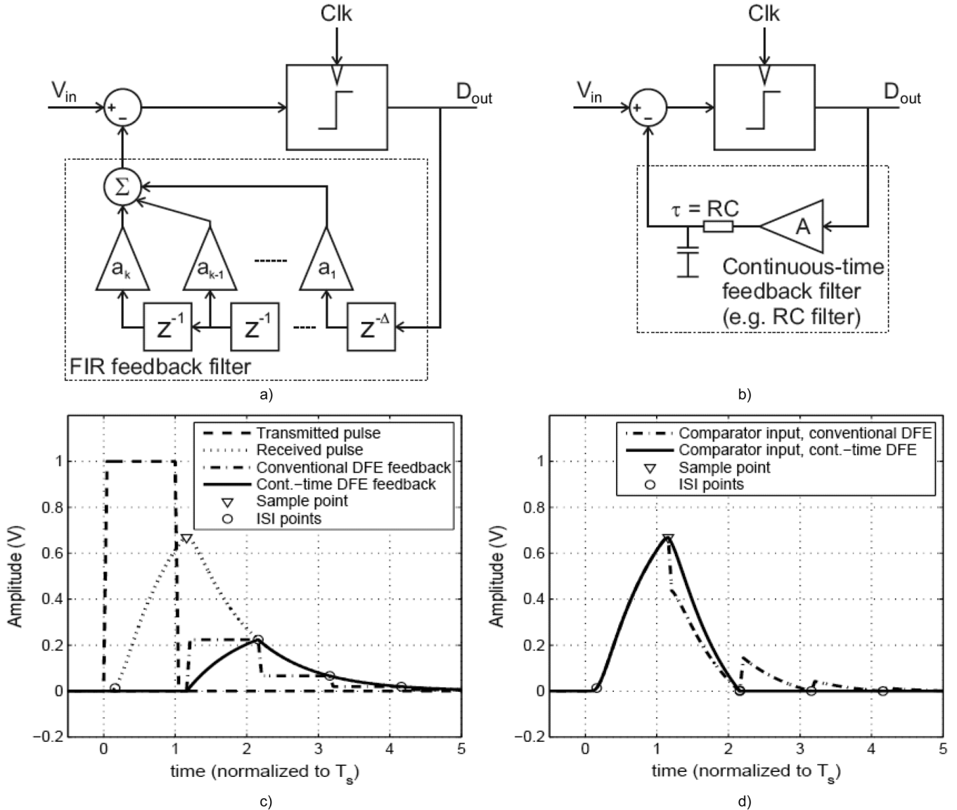
Fig. 7. Circuit diagram and simulated bit response for decision feedback equalization (DFE) with a discrete-time feedback filter (circuit a \Leftrightarrow response c) or a continuous-time (analog) feedback filter (circuit b \Leftrightarrow response d).
